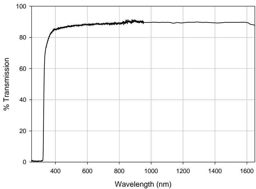
L2061-B 125 micron free-standing film
