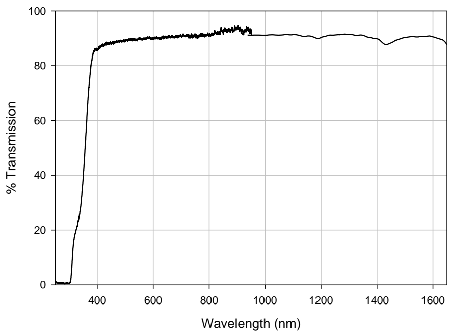
L2007 225 micron free-standing film
