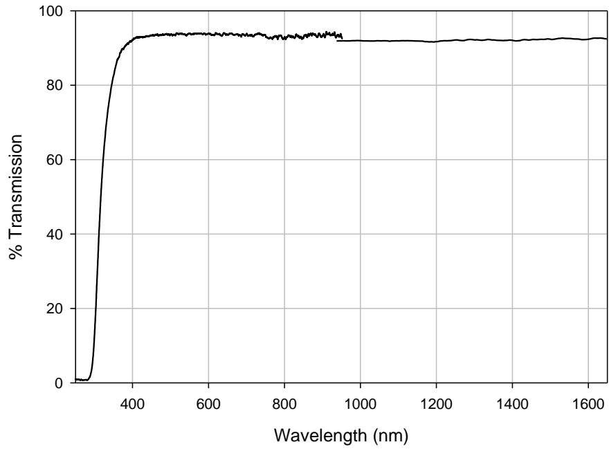
A200 20 micron cured film between glass substrates
